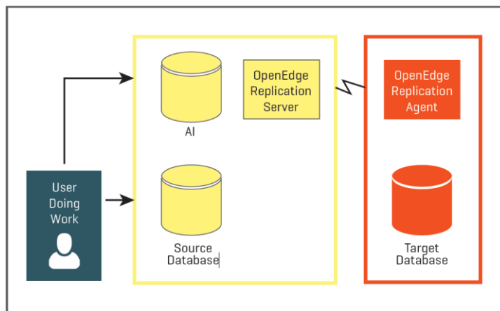
Рисунок 1 Source and Target Databases in OpenEdge Replication Model
